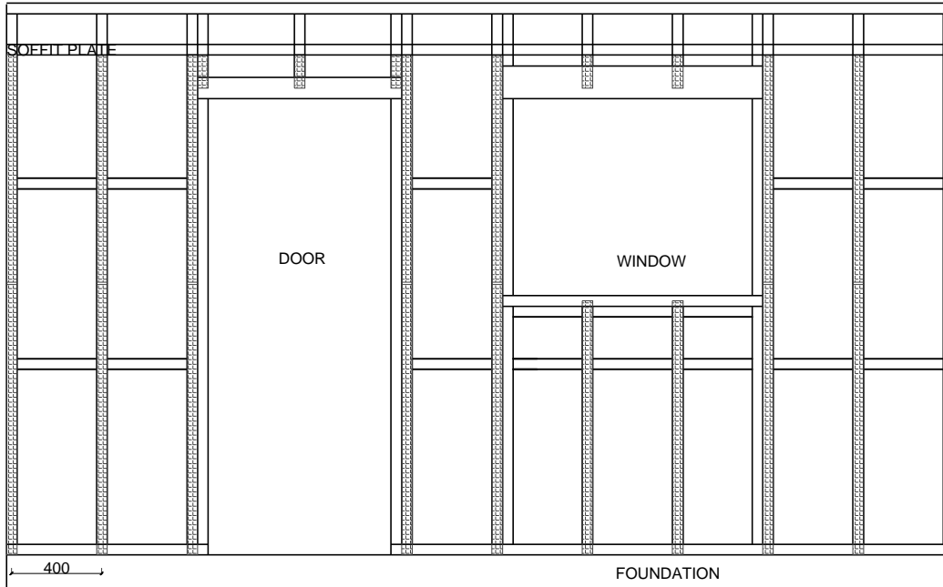
FRAMING STUDS 400mm CENTERS
