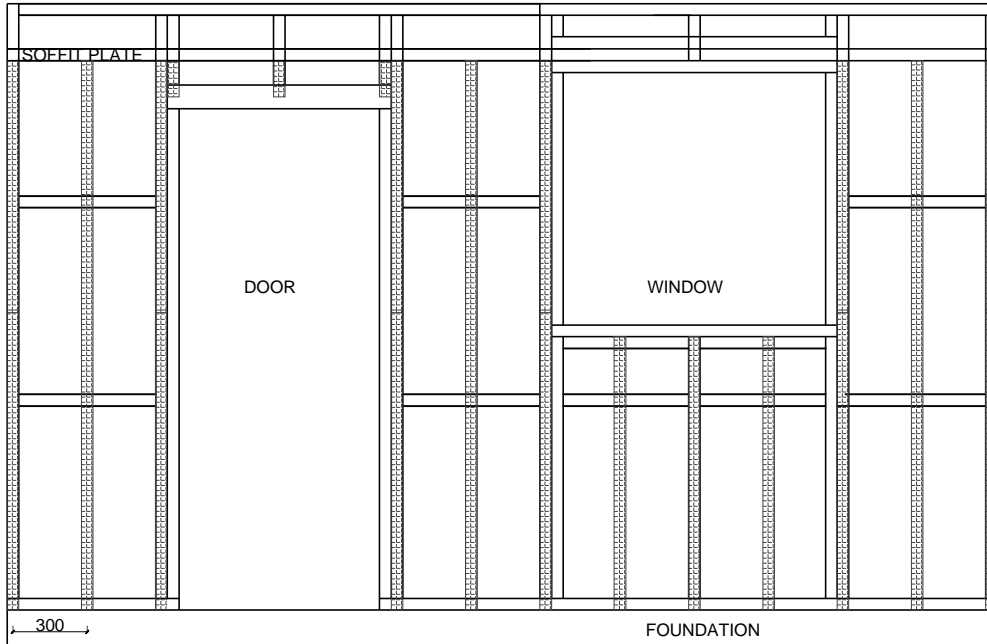
FRAMING STUDS 600mm CENTERS - WITH BATTENS @ 300mm CTRS
